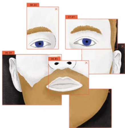
FACE DETECTION
