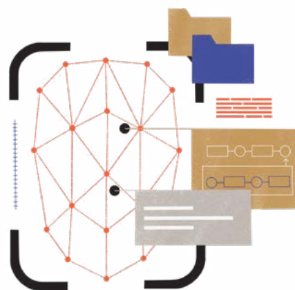
FACE MATCHING
