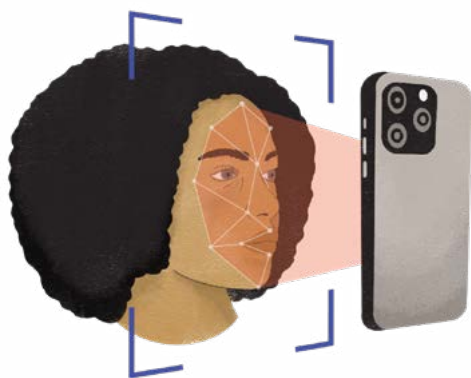
VERIFICATION
