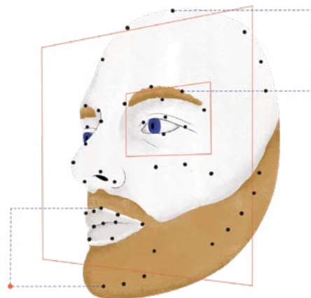
FACE ALIGNMENT
